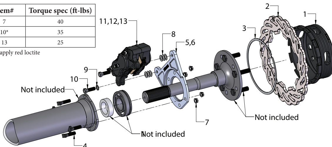
FIGURE # 1: Exploded B1706WCE Assembly View
